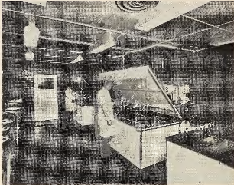
Festival's new plating department incorporating the latest design in nickel electroforming techniques with continuous solution treatment, air conditioning etc.
